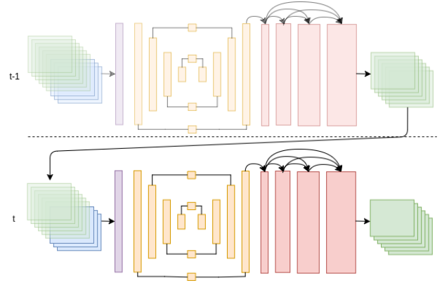
FIGURE 2 – Overview of our method for video face parsing. Blue channels : RGB facial image, Green channels : Mask predictions, More transparency signifies earlier predictions in time dimension. The output predictions of t - 1 is reinjected to t for robustness. Purple block : convolutional layer + batch norm layer. Yellow blocks : The Hourglass model composed of Mobile-net Blocks. Red blocks : Dense[4] Blocks
